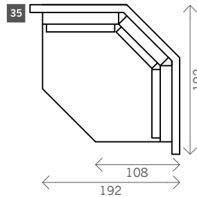
Corner XXL 2 wings
