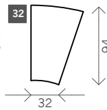
Corner XXL 2 wings
